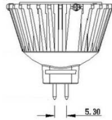
GU5.3
